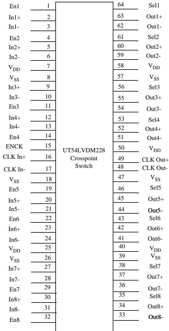
Figure 2. UT54LVDS228 Pinout
