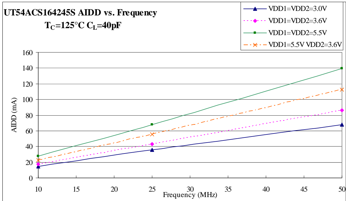
Figure 4. AIDD Values for 125^\circ\text{C} with all 16 outputs switching
