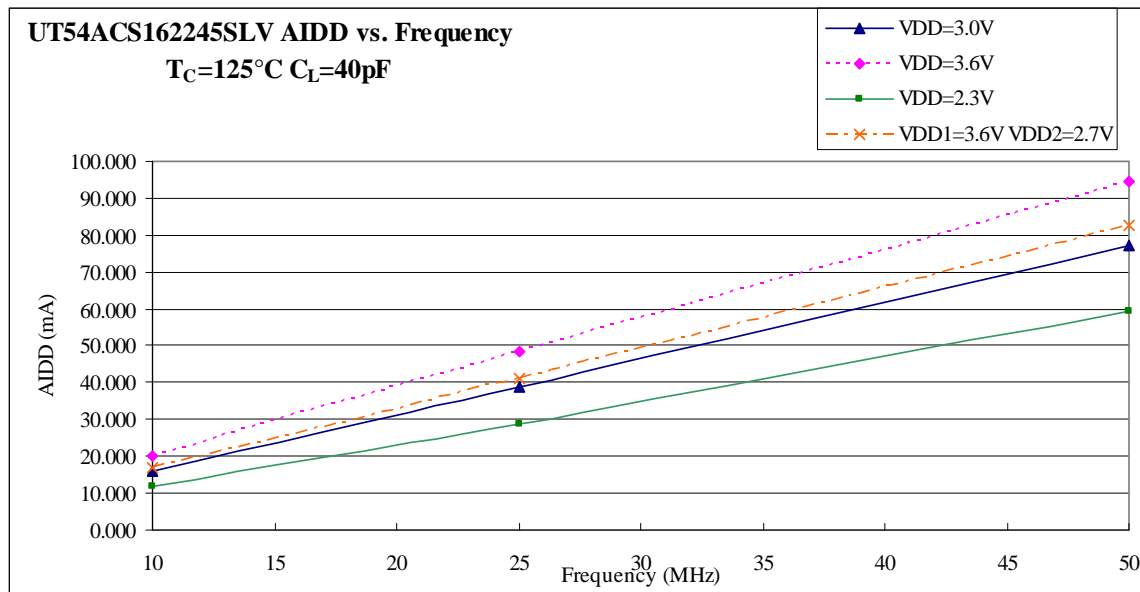
Figure 10. AIDD Values for 125^\circ\text{C} with all 16 outputs switching
