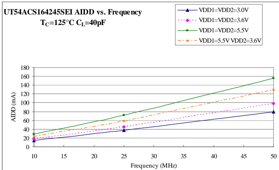
Figure 1. AIDD Values for 125^\circ\text{C} with all 16 outputs switching
