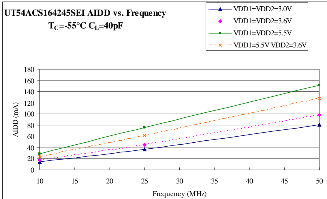
Figure 3 AIDD Values for -55^\circ\text{C} with all 16 outputs switching
