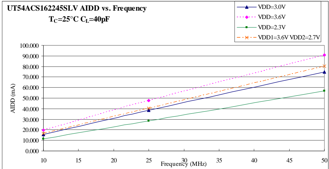
Figure 11. AIDD Values for 25^\circ\text{C} with all 16 outputs switching
