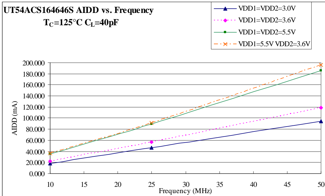
Figure 7. AIDD Values for 125^\circ\text{C} with all 16 outputs switching
