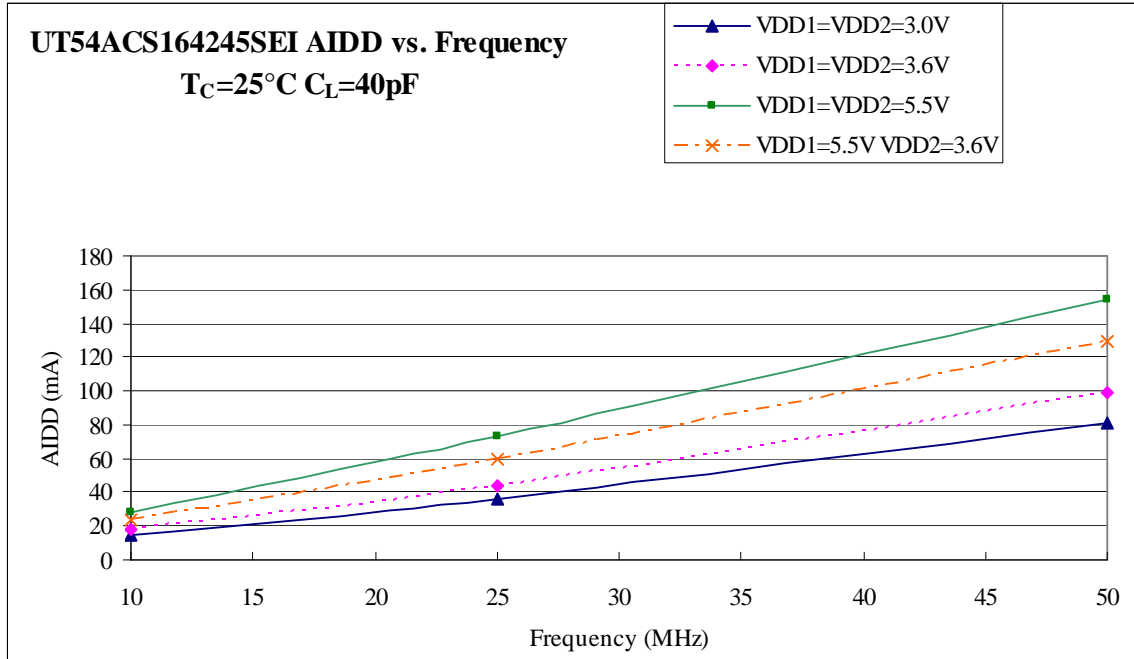
Figure 2. AIDD Values for 25^\circ\text{C} with all 16 outputs switching
