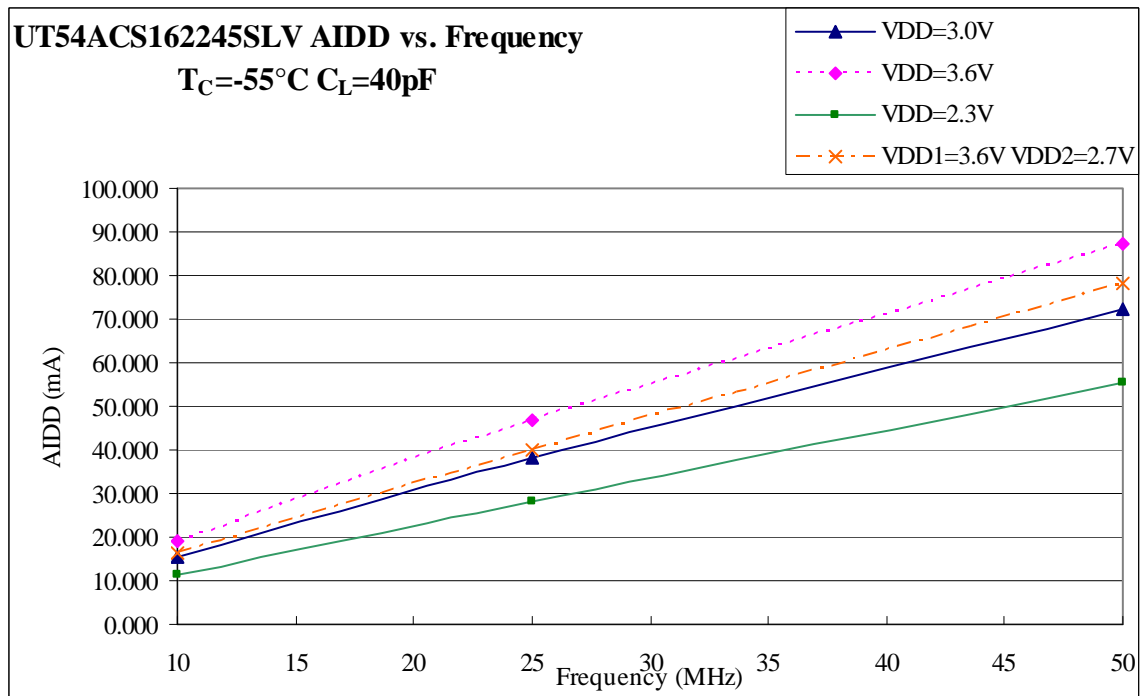
Figure 12. AIDD Values for -55^\circ\text{C} with all 16 outputs switching
