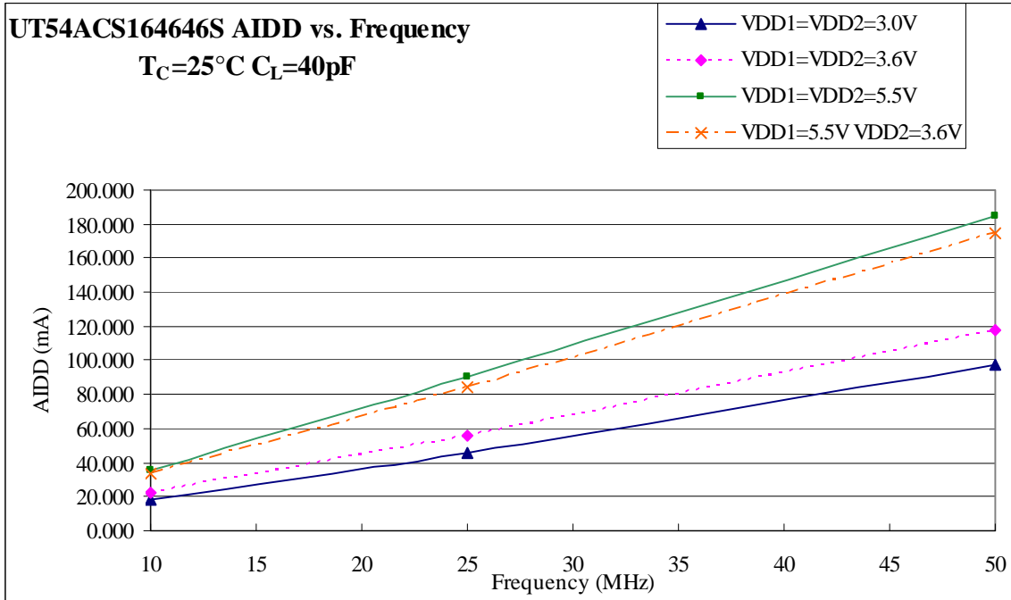
Figure 8. AIDD Values for 25^\circ\text{C} with all 16 outputs switching
