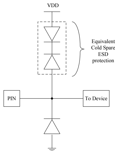
Figure 1. Notional Cold Spare ESD protection circuit
