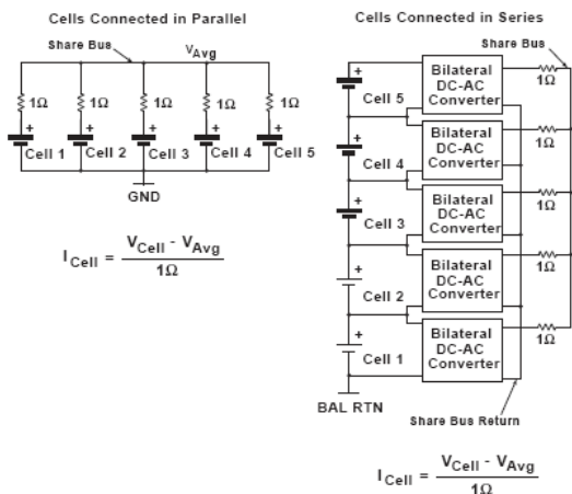
Figure 1 - Cell Balancing by Share Bus
