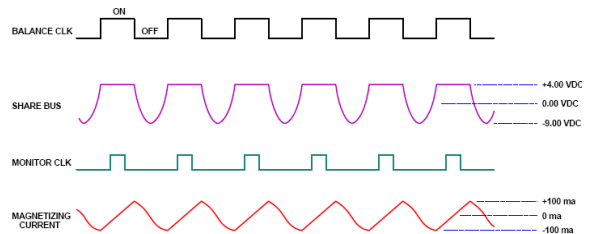
Figure 3 - Cell Balancing Timing Diagram
