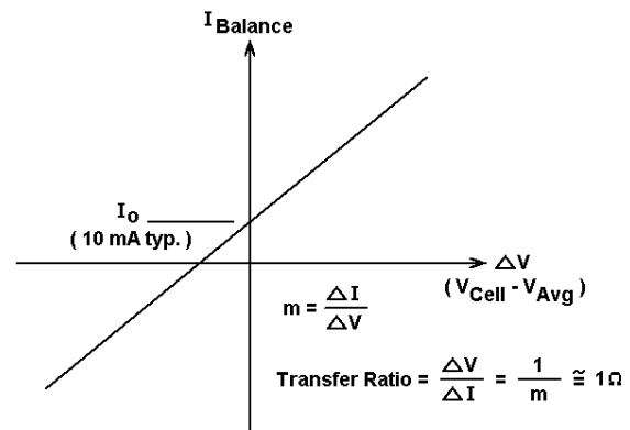
Figure 5 - Cell Balancing Characteristic Curve
