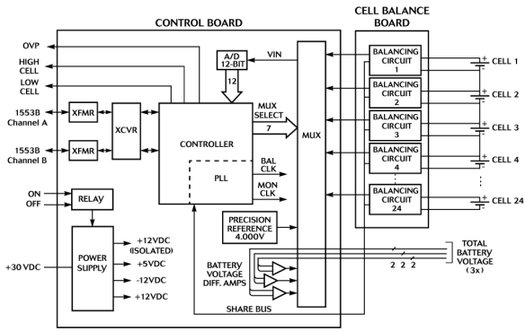
Figure 4 - BEU Functional Block Diagram (Single Channel)
