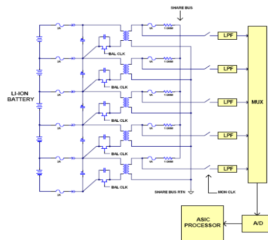
Figure 2 - Cell Balancing Circuit
