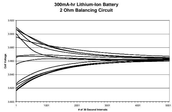
Figure 9 - Balancing of 13 Cell Battery
