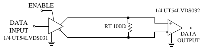
Figure 3. Point-to-Point Application
