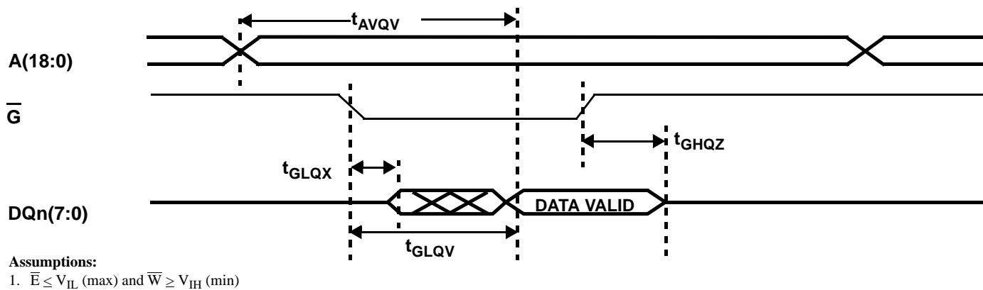
Figure 3c. SRAM Read Cycle 3: Output Enable-Controlled Access
