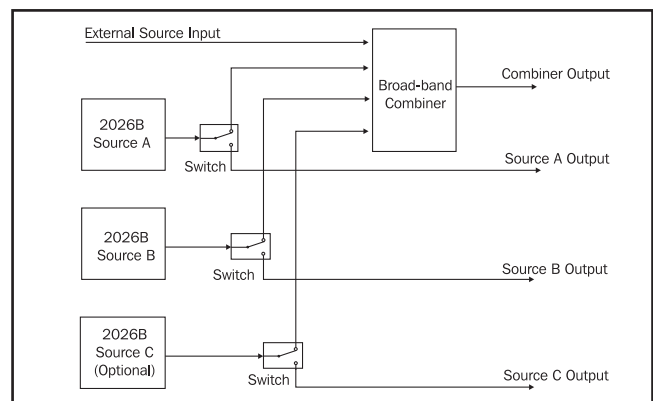
Figure 2 - 2026B block diagram
