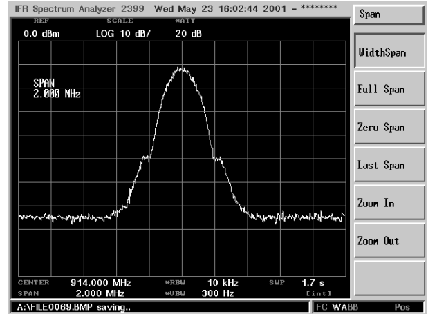
Figure 6 - 2026B Opt. 117 GSM signal emulation
