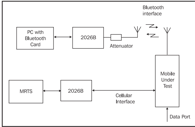
Figure 4 - Using 2026B to aid testing the Bluetooth and GSM air interfaces
