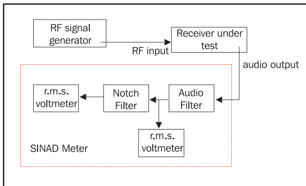
Figure 1-SINAD measurement system
