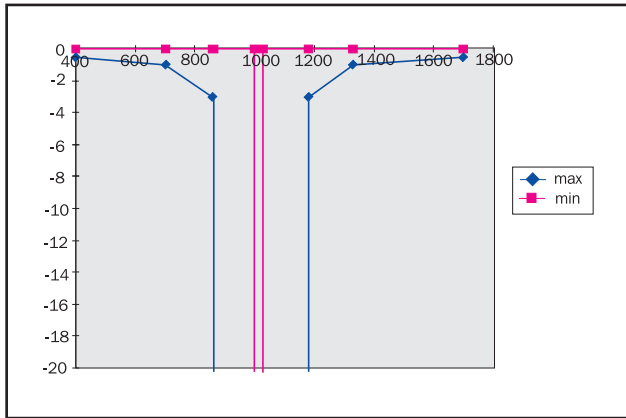
Figure 4 - Limits for Notch Filter ITU-T 0.132
